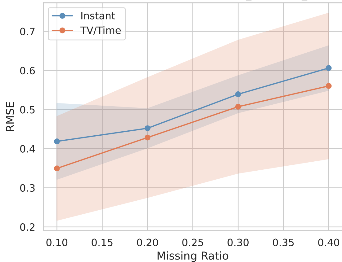
RMSE — TV/Time vs Instant — it05b_synthetic_three
