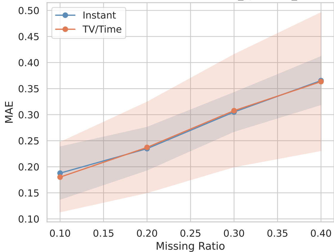
MAE — TV/Time vs Instant — it05b_synthetic_three
