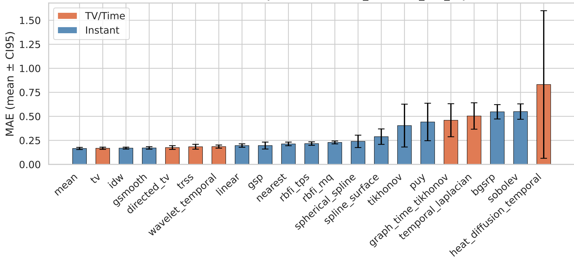
Mean Absolute Error by Method — it06b_kalofolias_nnk_3syn
