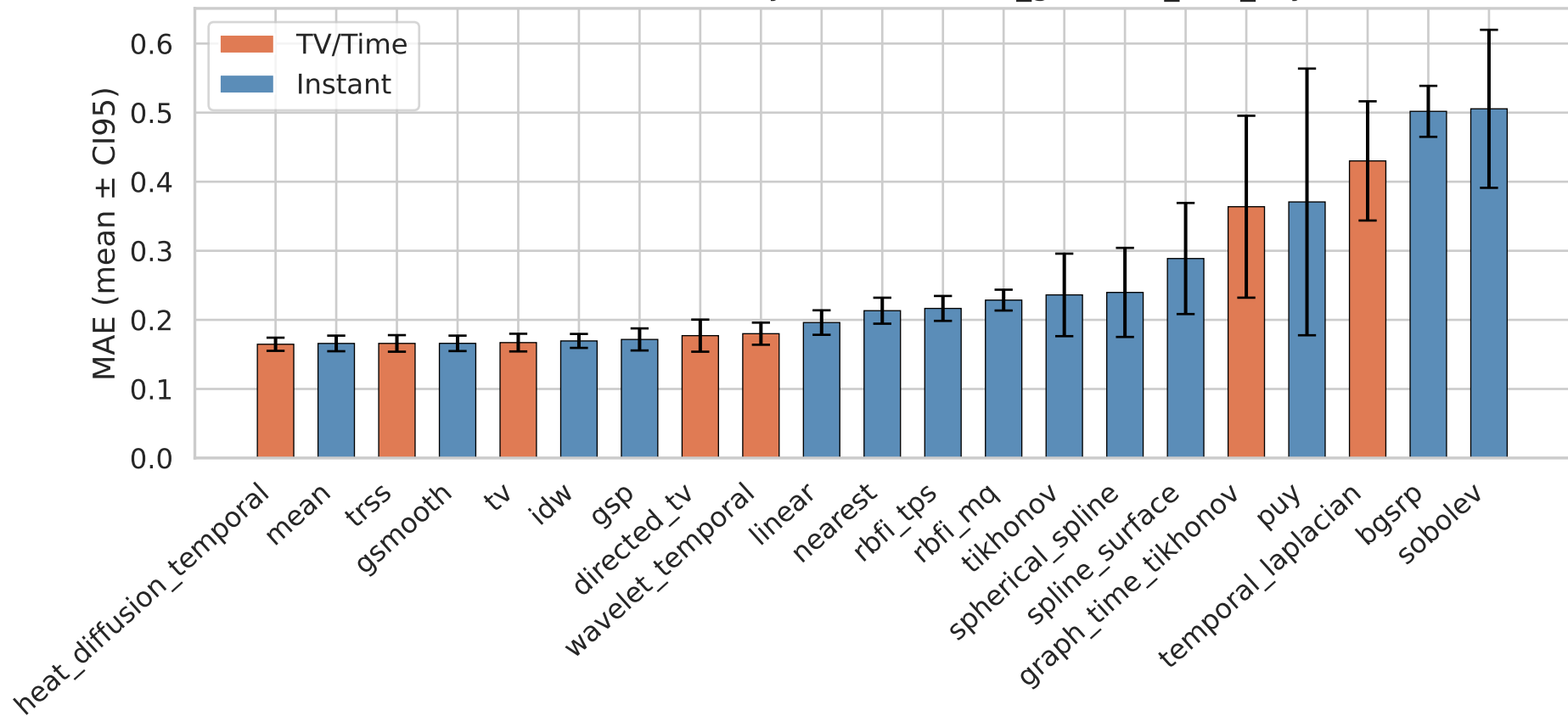
Mean Absolute Error by Method — it13_gaussian_aew_3syn
