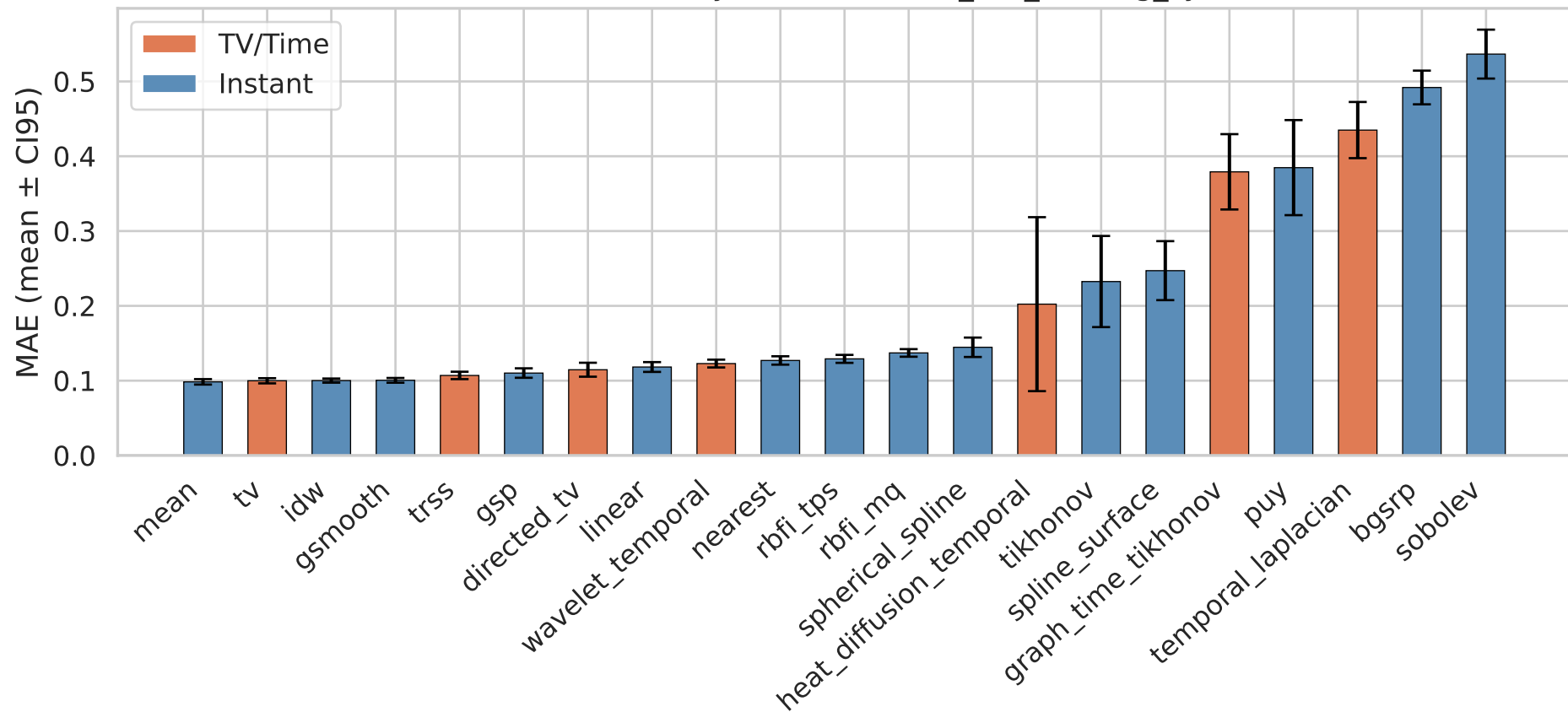
Mean Absolute Error by Method — it14_low_missing_synthetic
