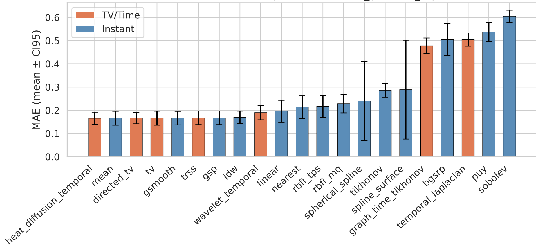
Mean Absolute Error by Method — it15b_gaussian_3syn
