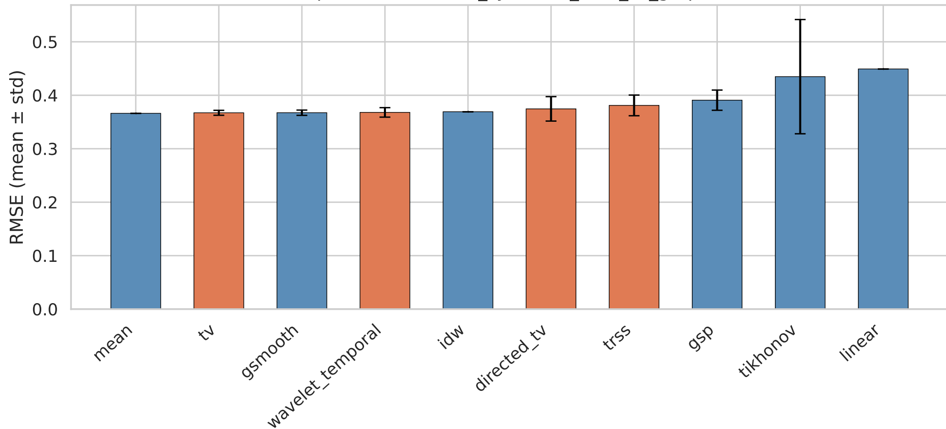
Top-10 RMSE — it26_synthetic_beta_all_graphs
