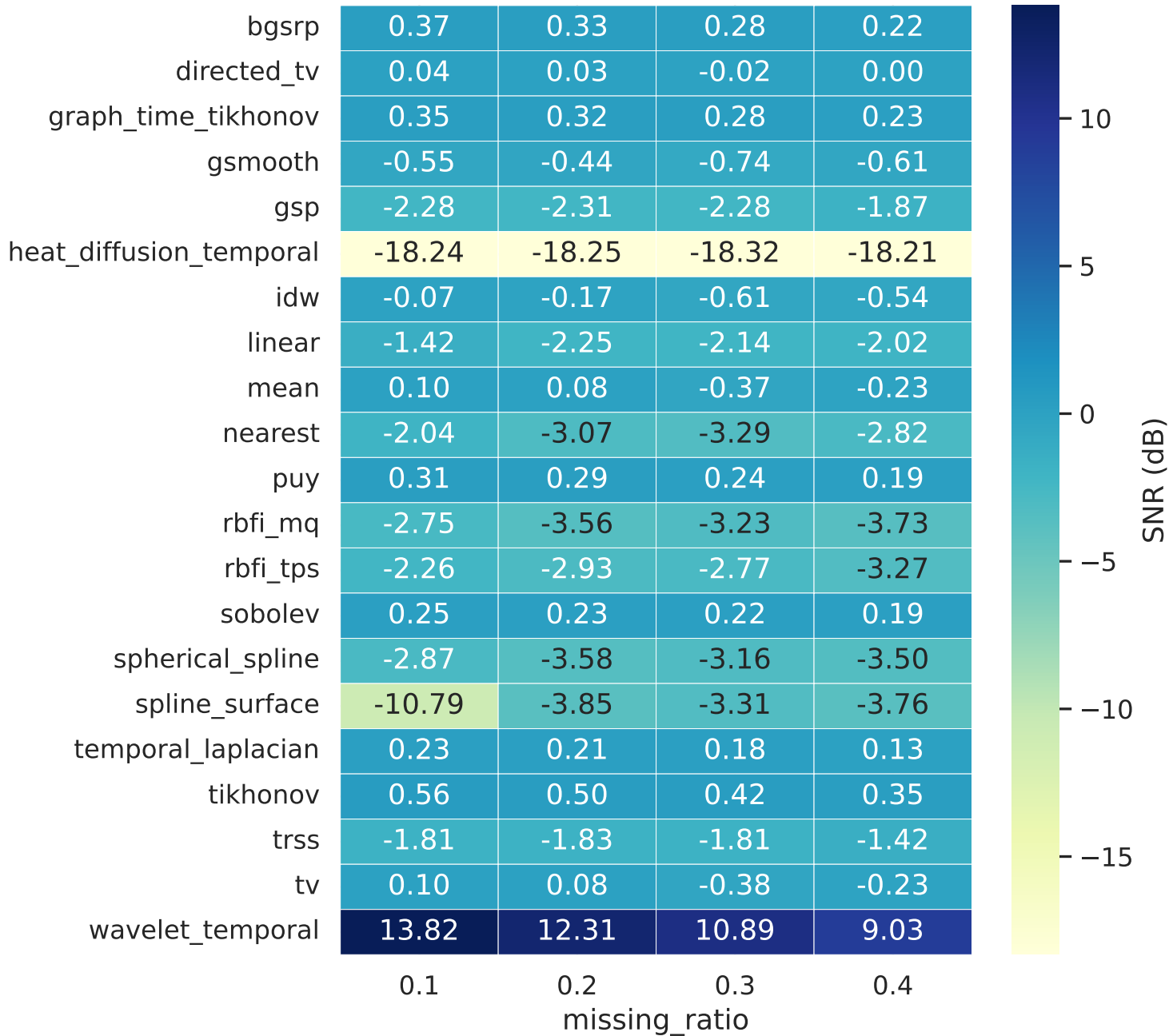
Mean SNR — Method × Scenario — it29_kalofolias_3syn
