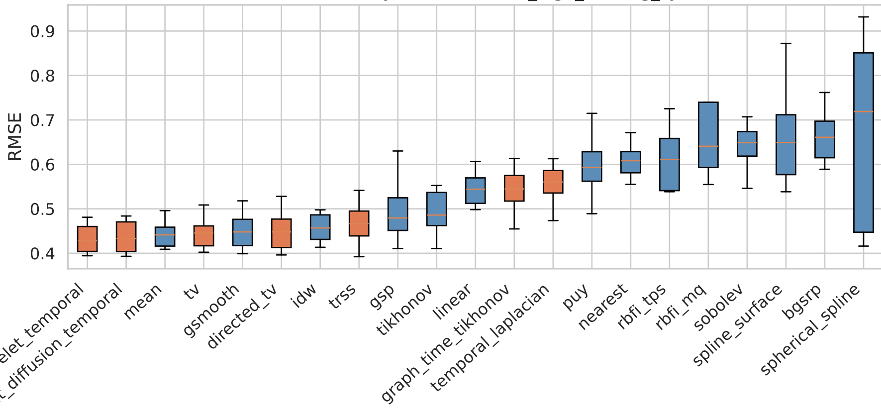
RMSE Distribution by Method — it08_high_missing_synthetic
