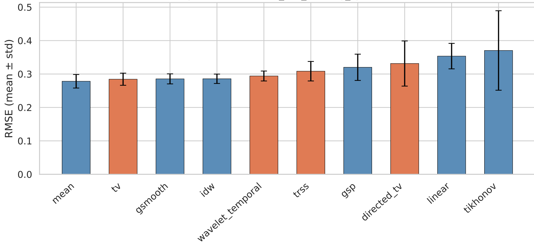
Top-10 RMSE — it14_low_missing_synthetic
