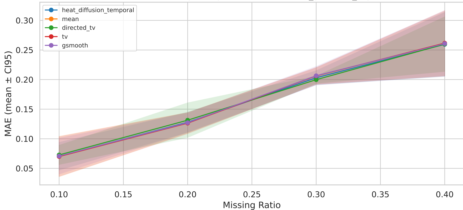
MAE Sensitivity — Top-5 Methods — it15b_gaussian_3syn
