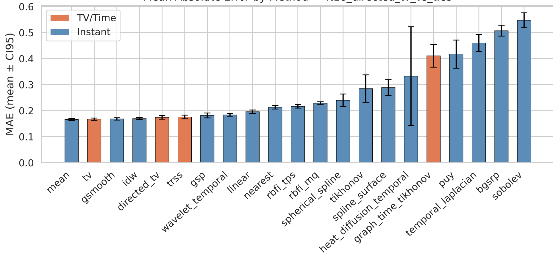
Mean Absolute Error by Method — it18_directed_tv_vs_trss
