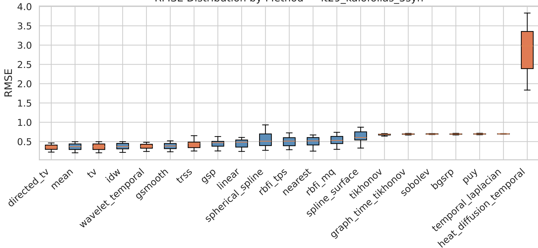
RMSE Distribution by Method — it29_kalofolias_3syn
