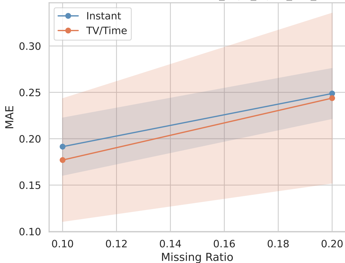
MAE — TV/Time vs Instant — it37_3syn_alpha_low_missing
