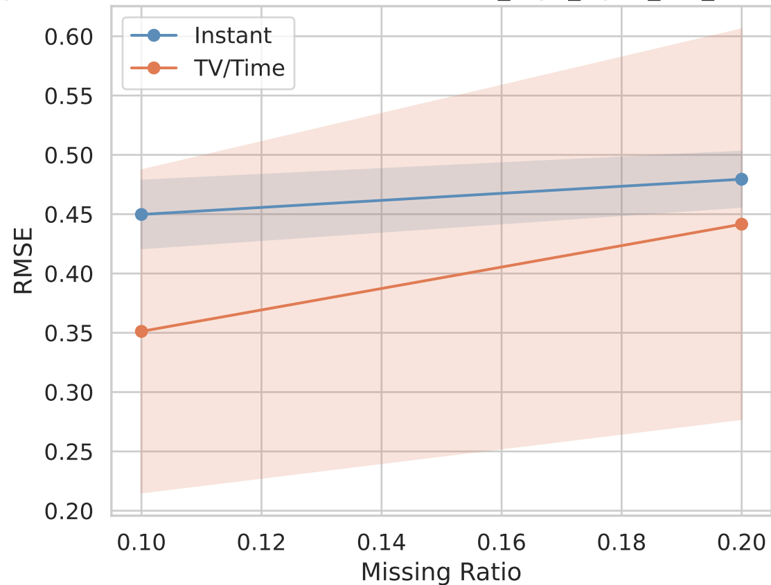
RMSE — TV/Time vs Instant — it37_3syn_alpha_low_missing
