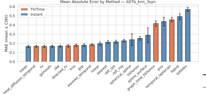
Fig. 6. MAE mean \pm CI95 per method — iteration it07b\_knn\_3syn . Orange: TV/Time family; blue: Instant family.
