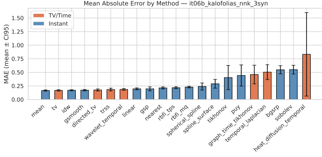
Fig. 5. MAE mean \pm CI95 per method — iteration it06b\_kalofolias\_nnk\_3syn . Orange: TV/Time family; blue: Instant family.
