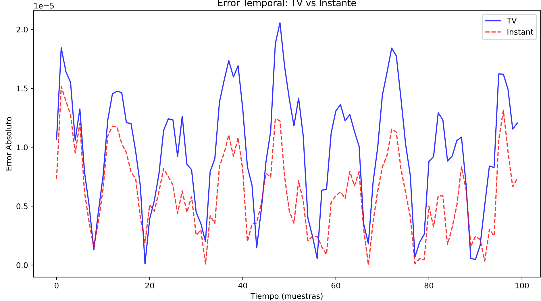
it77_few_missing_bci_all_graphs
