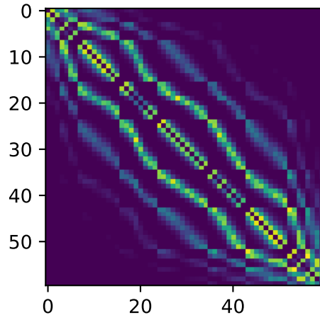
Sklearn Radius
