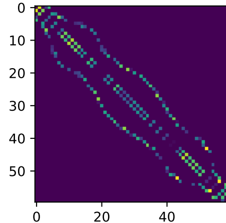
NNK
