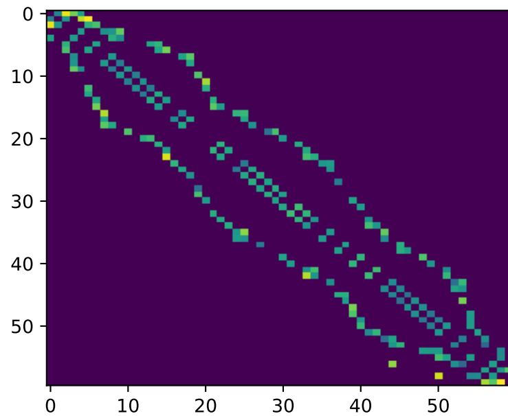
AEW
