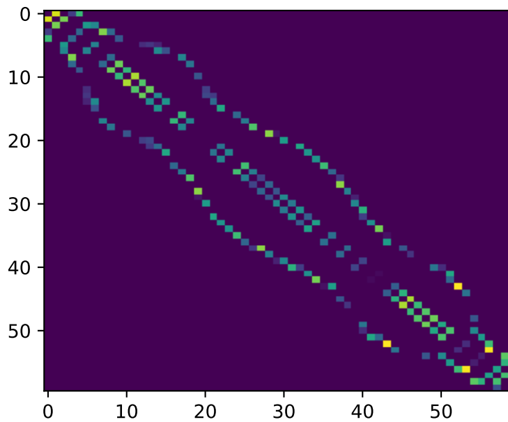
NNK
