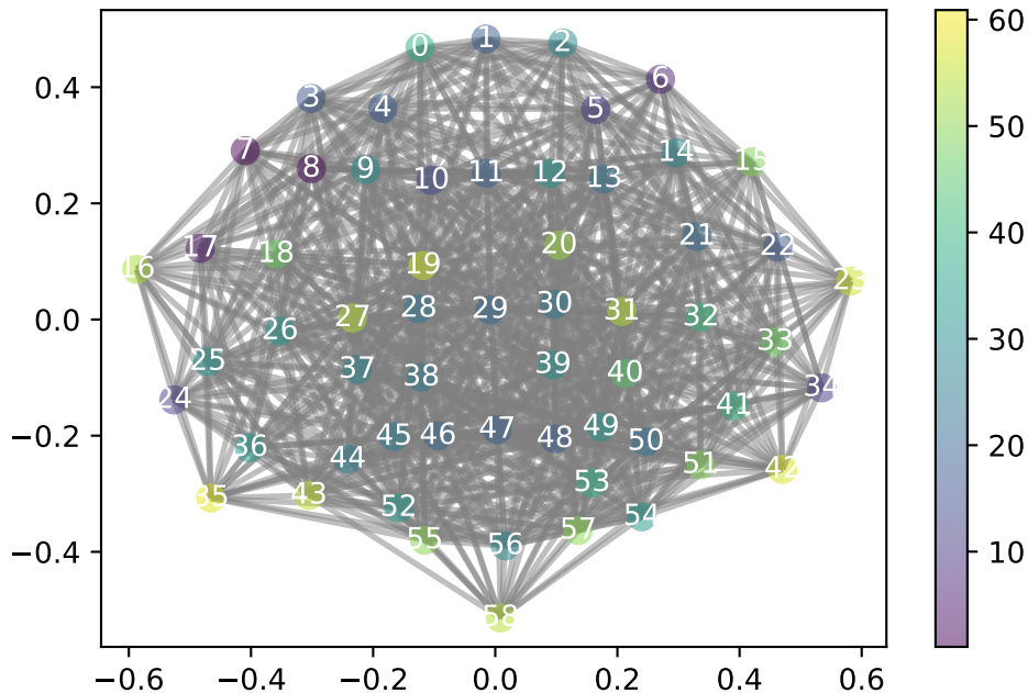
Problem idxs
