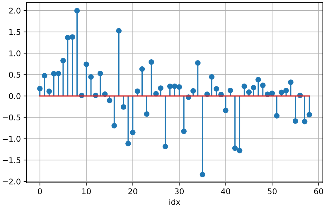
Error_rbf-error_method_by_idx
