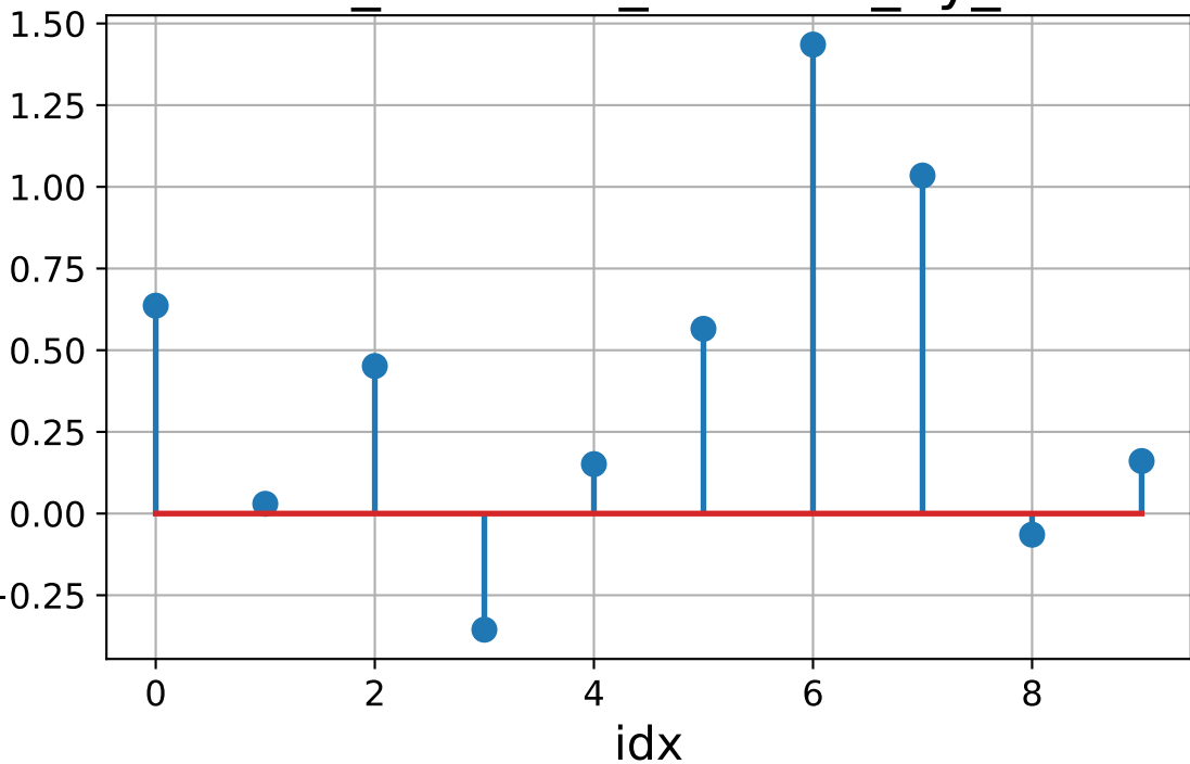
Error_rbi-error_method_by_idx
