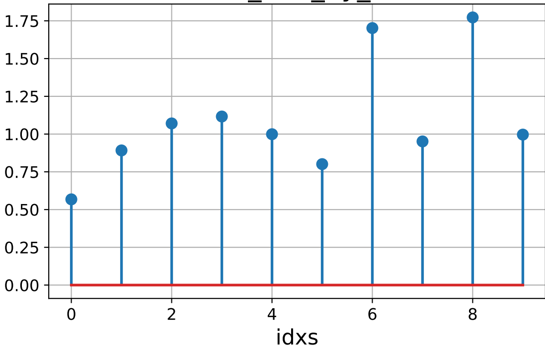
error_min_by_idx
