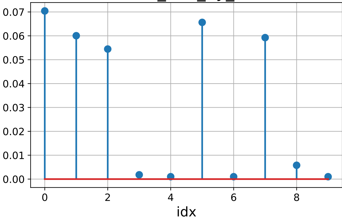
theta_min_by_idx
