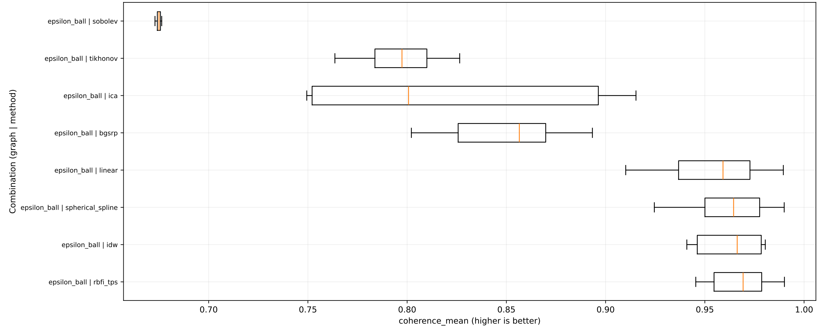
coherence_mean distribution by graph-method combination - dataset: mne_sample
