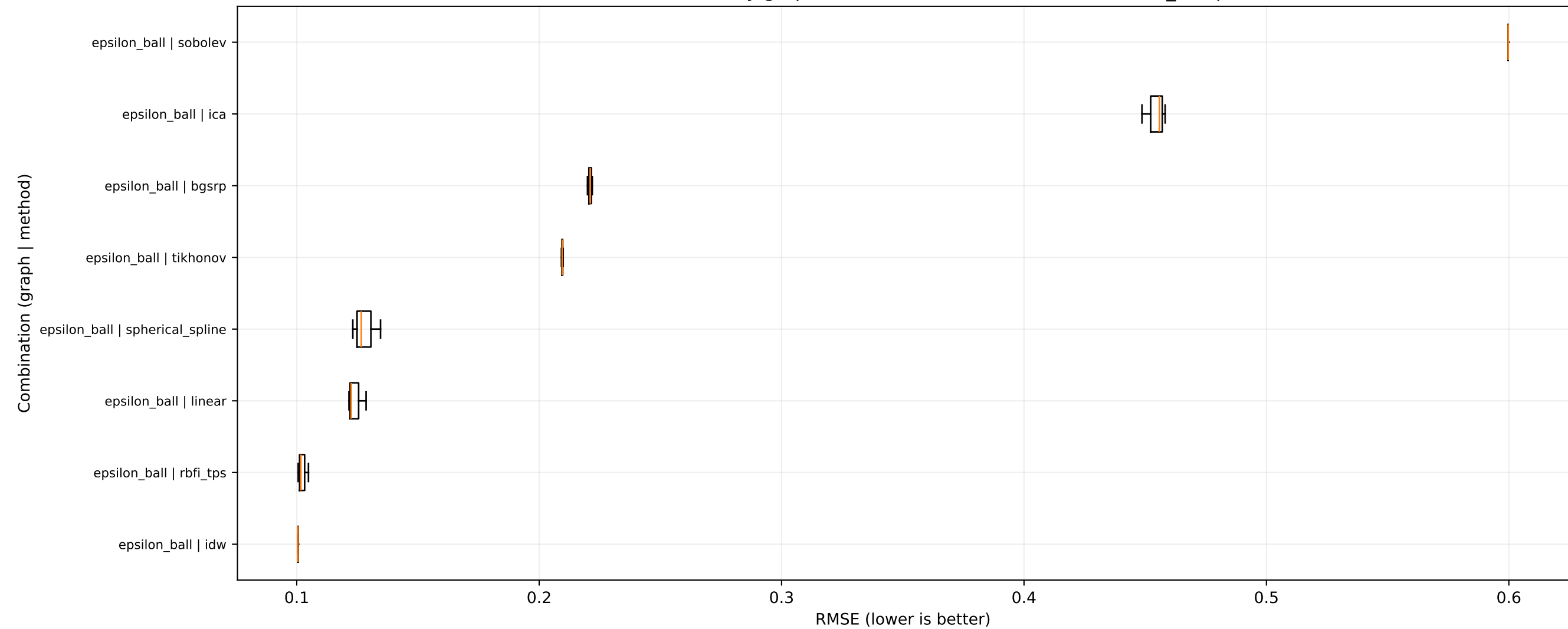
RMSE distribution by graph-method combination - dataset: mne_sample
