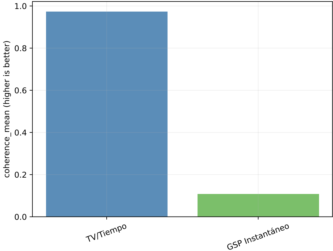
coherence_mean
