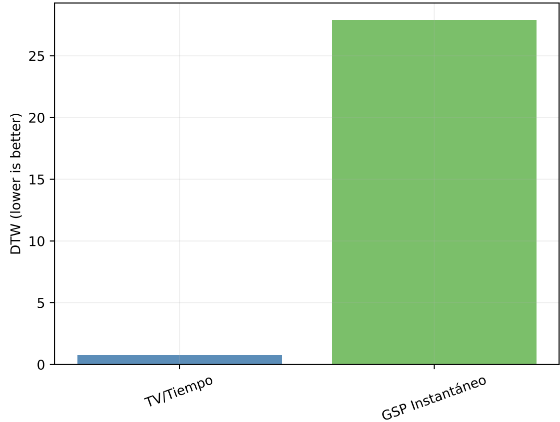
DTW
