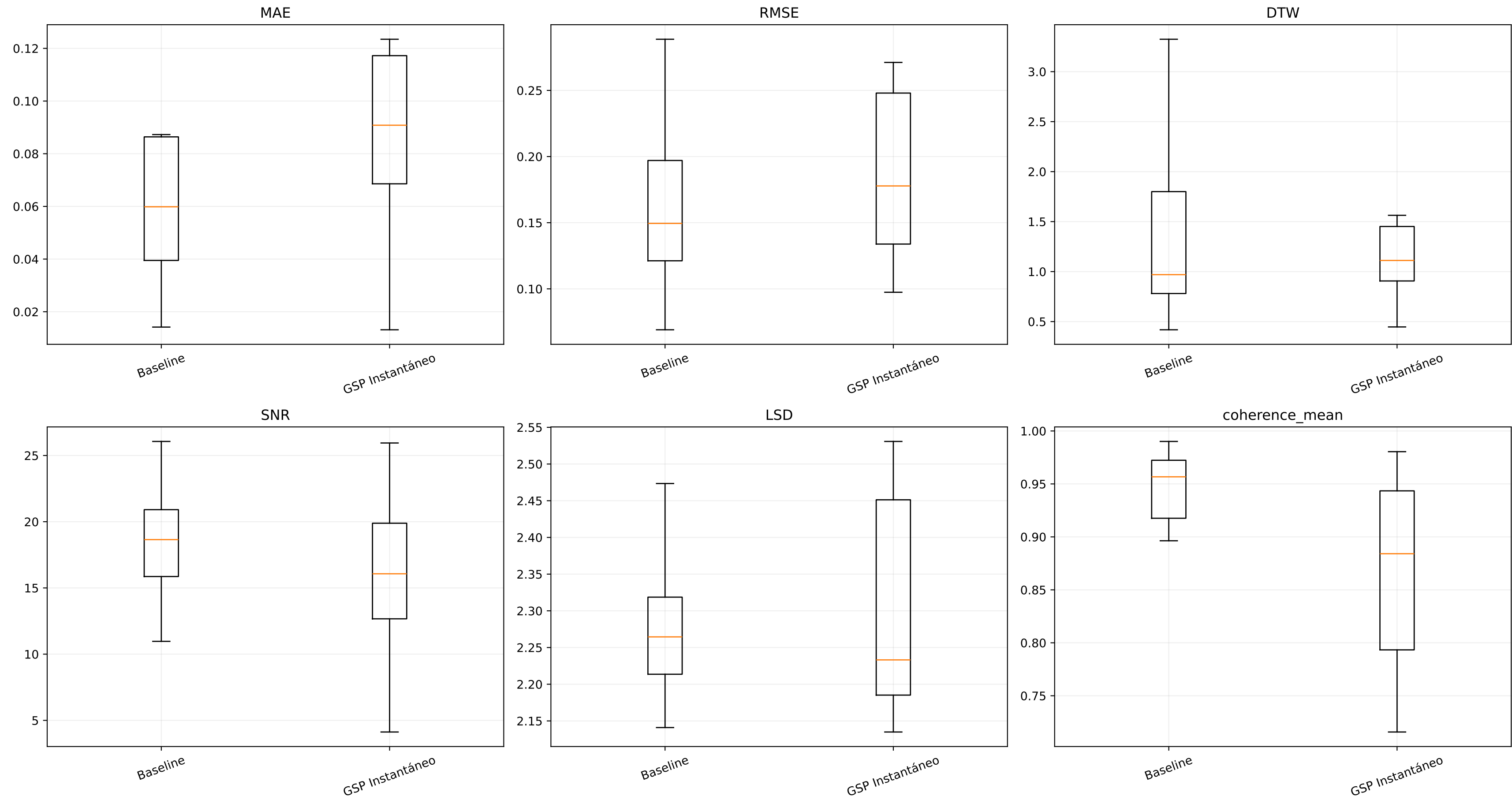
Family dispersion by metric - dataset: mne_sample
