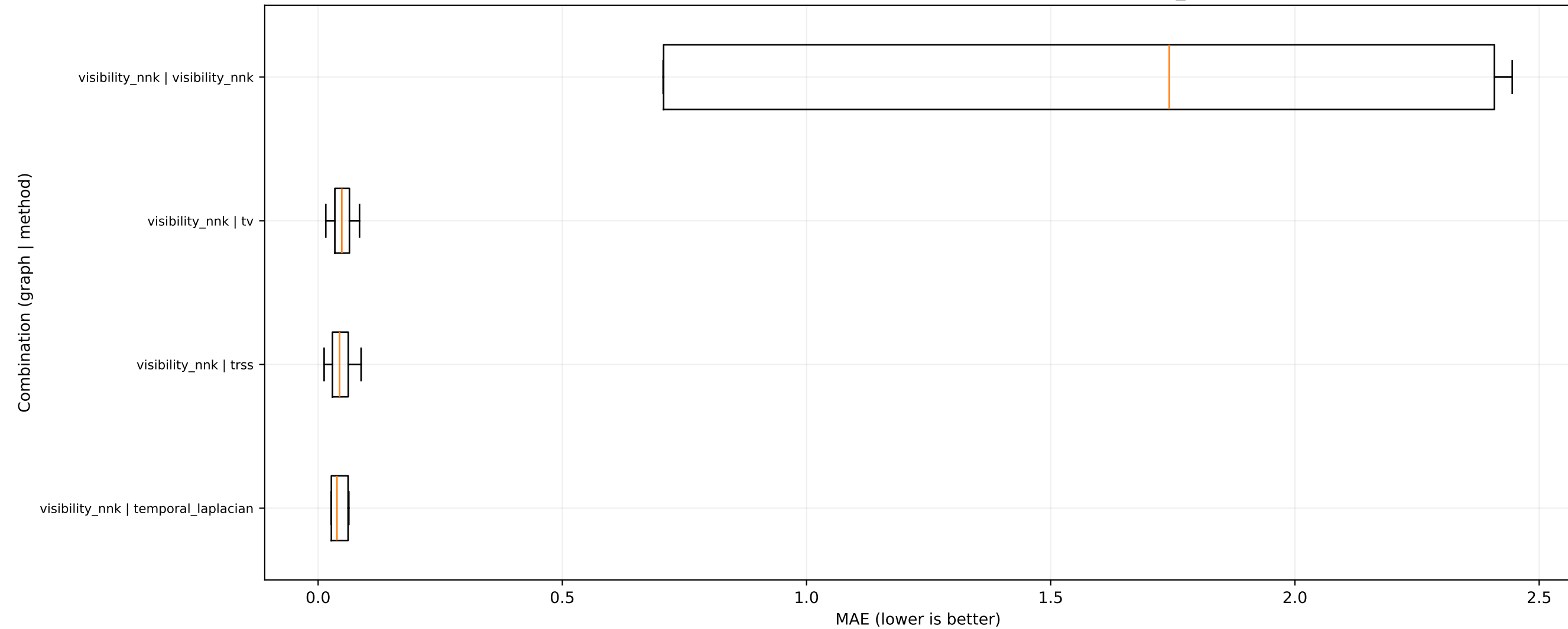
MAE distribution by graph-method combination - dataset: mne_sample
