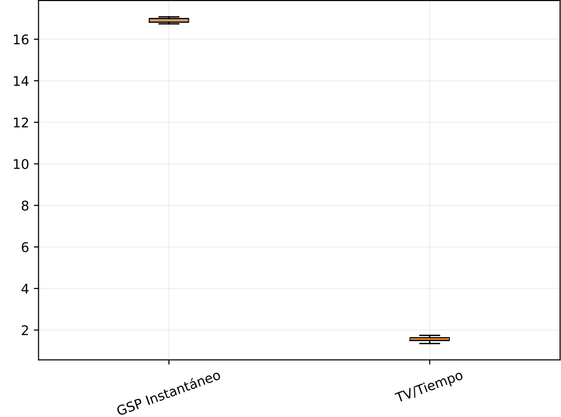
coherence_mean
