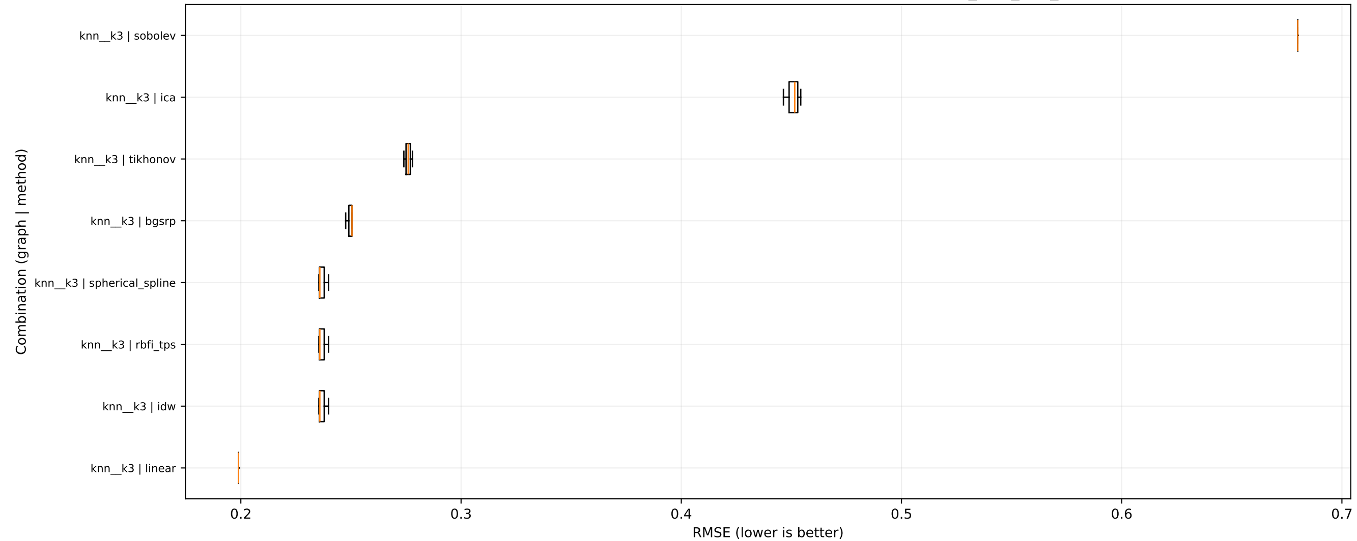
RMSE distribution by graph-method combination - dataset: bci_iv2a_real_s3
