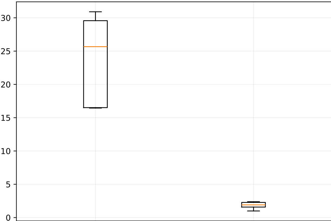
DTW
