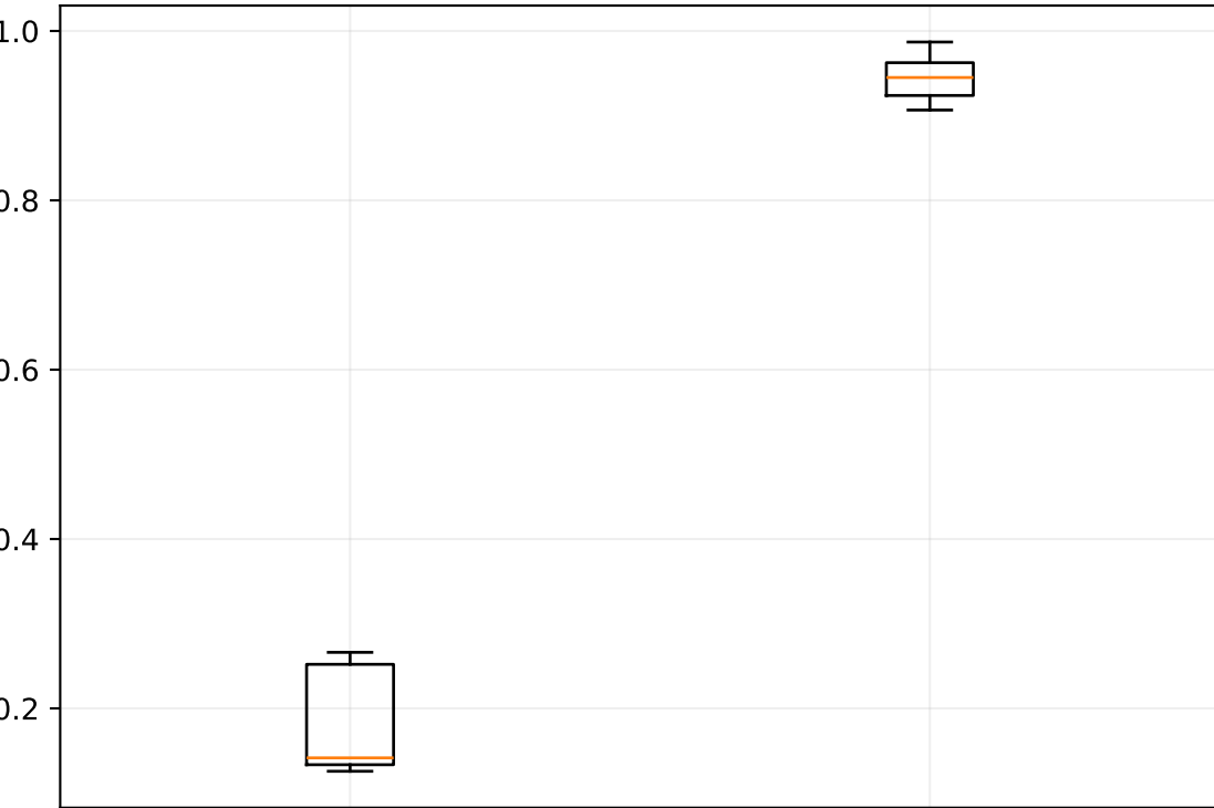
coherence_mean
