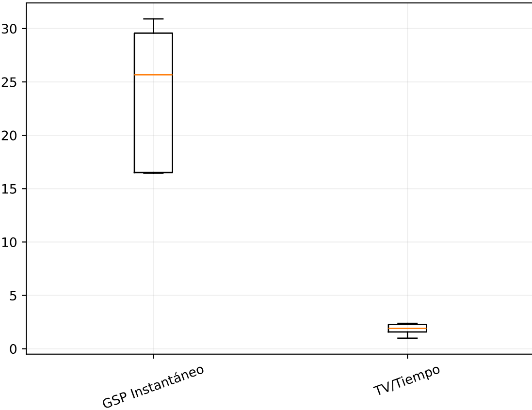
coherence_mean
