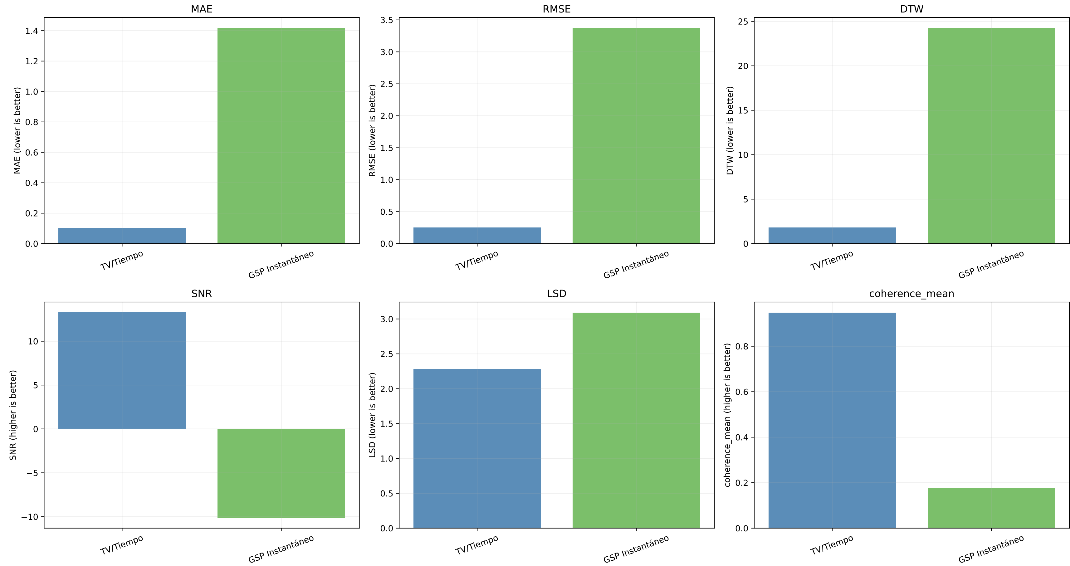
Average performance by family - dataset: bci_iv2a_real_s3
