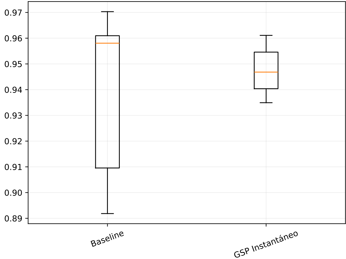
coherence_mean
