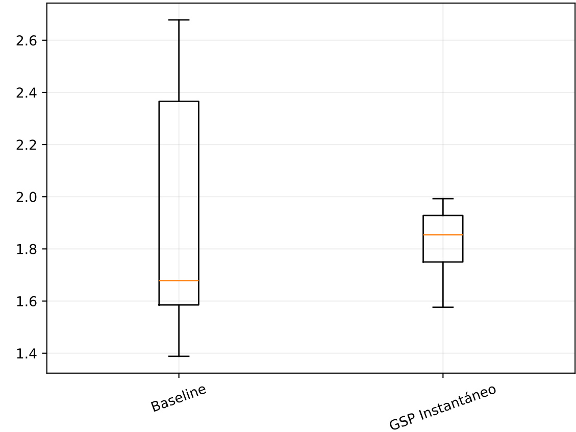
DTW
