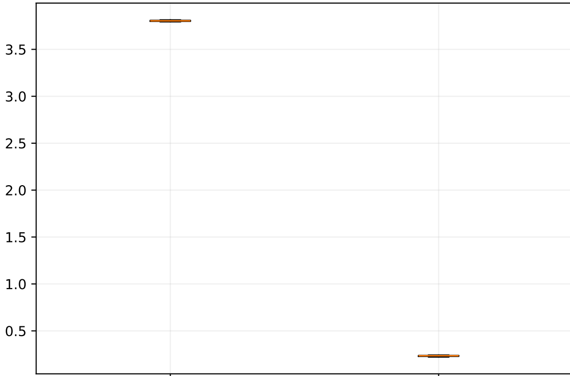
RMSE
