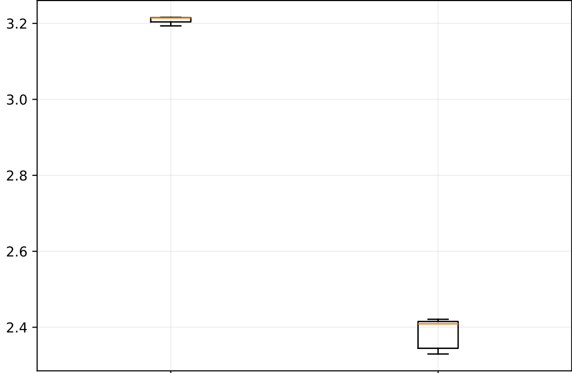
LSD
