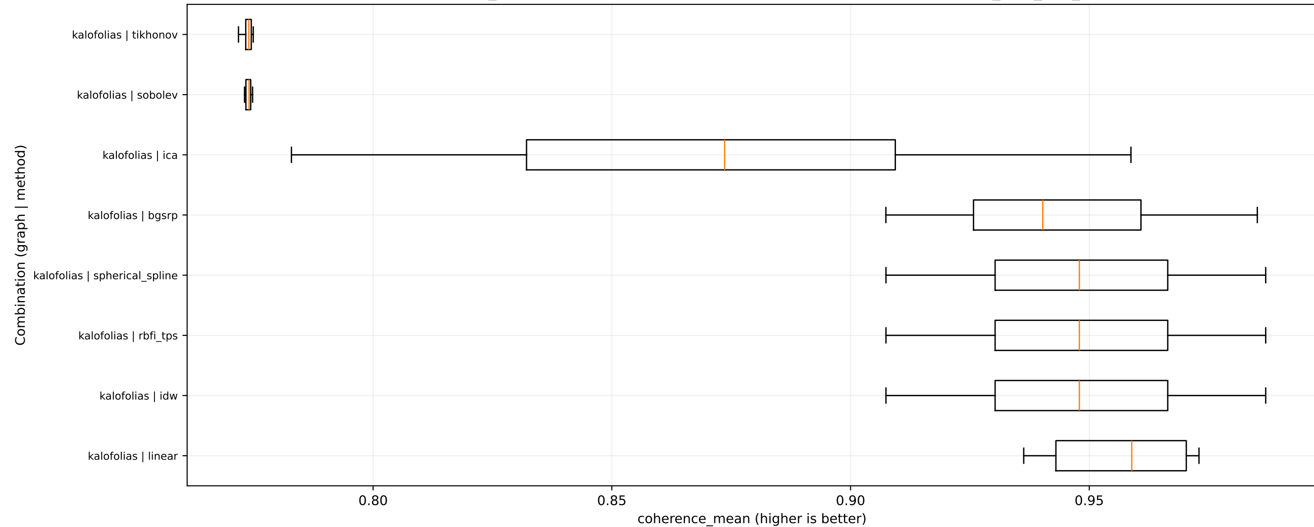
coherence_mean distribution by graph-method combination - dataset: bci_iv2a_real_s3
