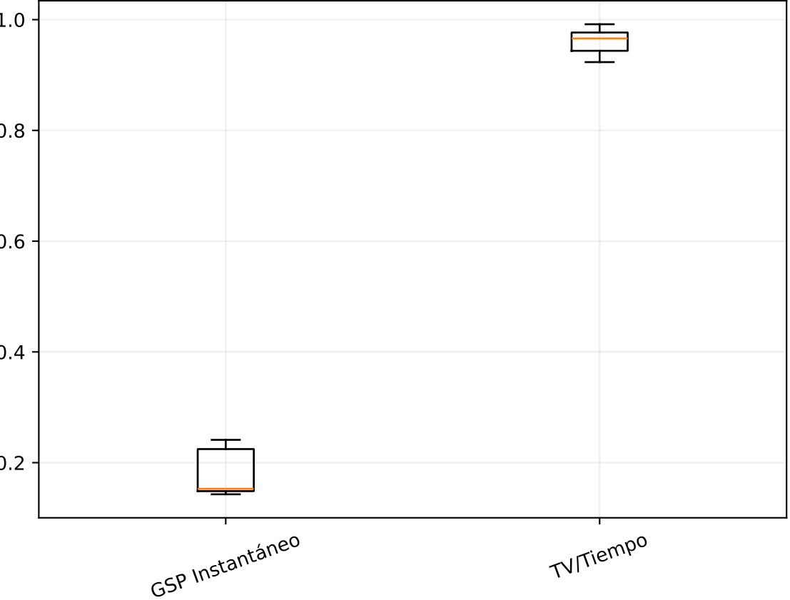
coherence_mean
