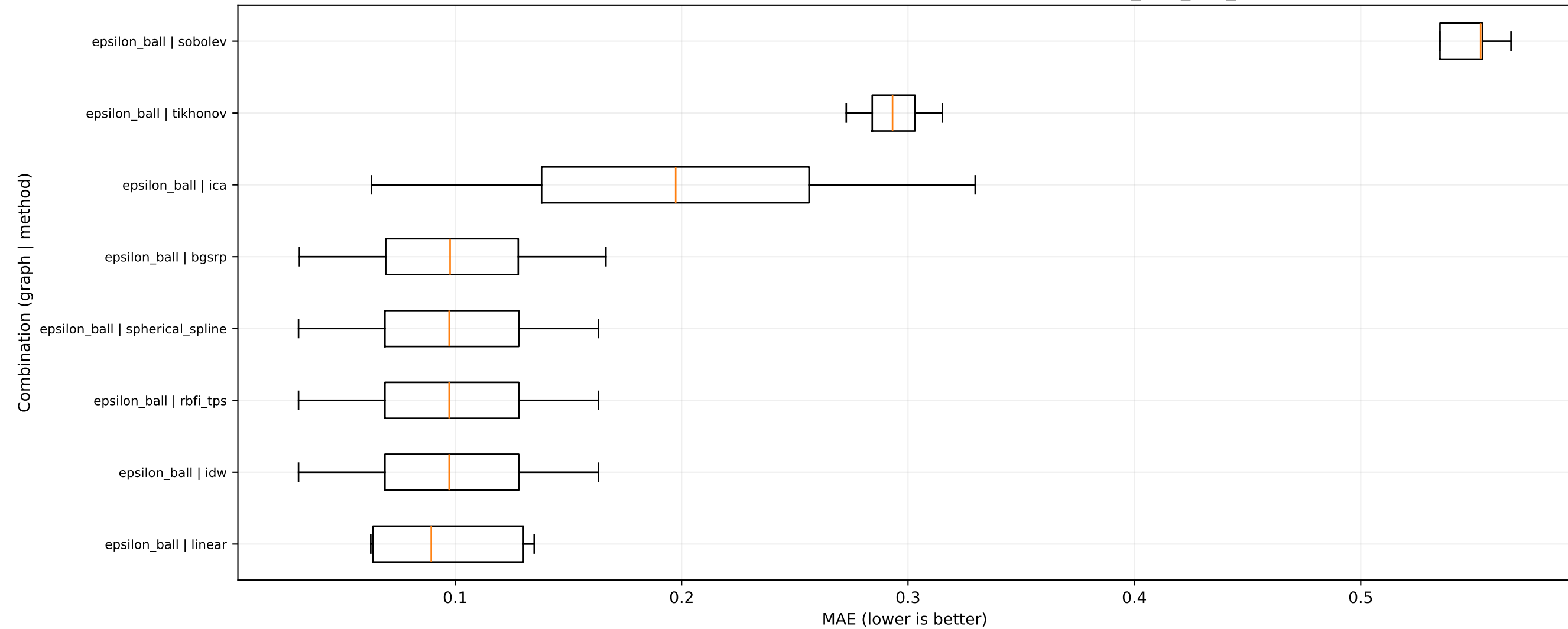
MAE distribution by graph-method combination - dataset: bci_iv2a_real_s3
