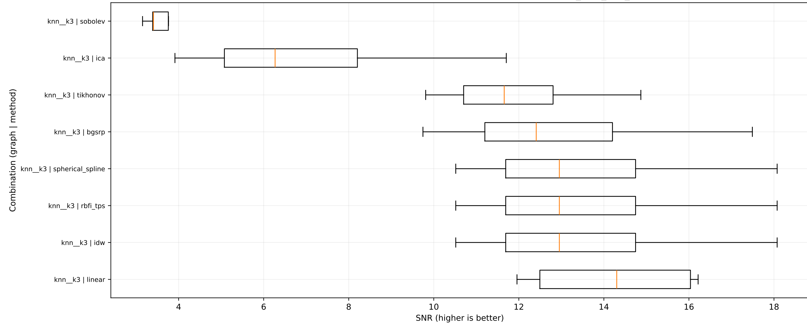
SNR distribution by graph-method combination - dataset: bci_iv2a_real_s3
