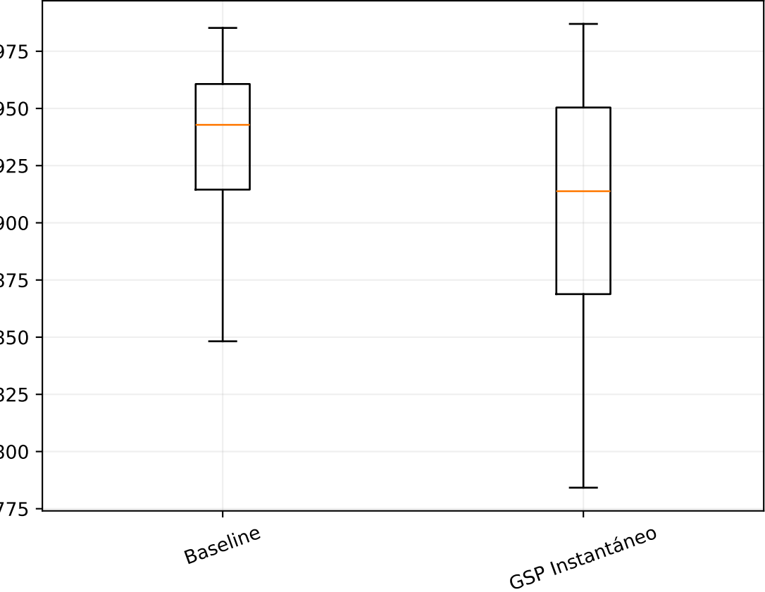
coherence_mean
