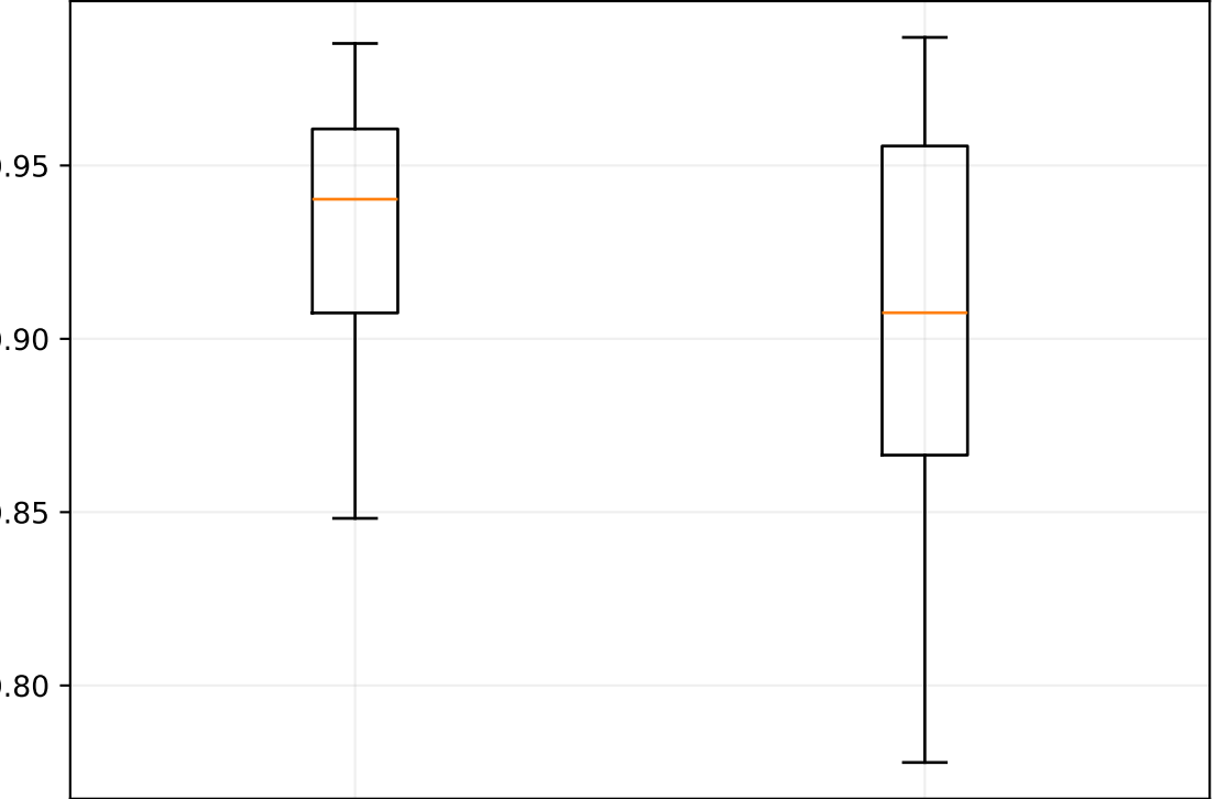
coherence_mean
