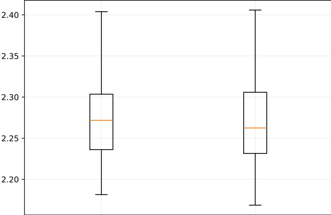
LSD
