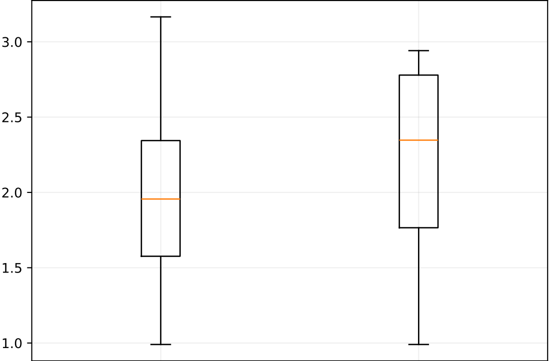
DTW
