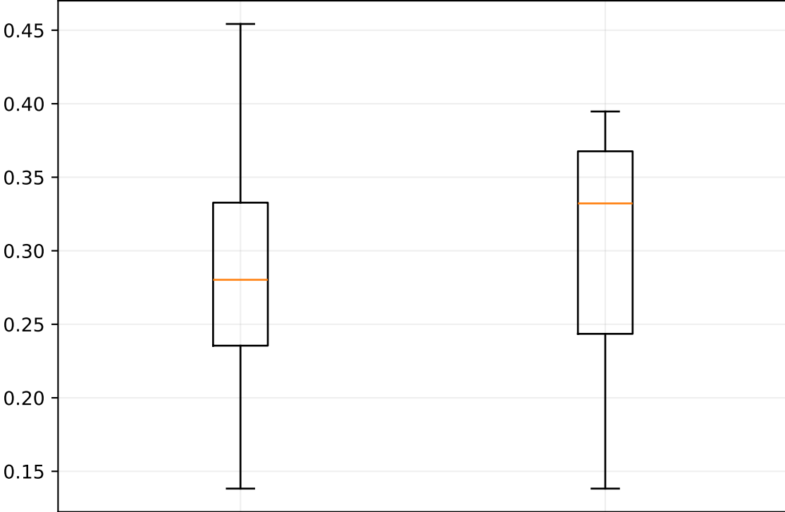
RMSE
