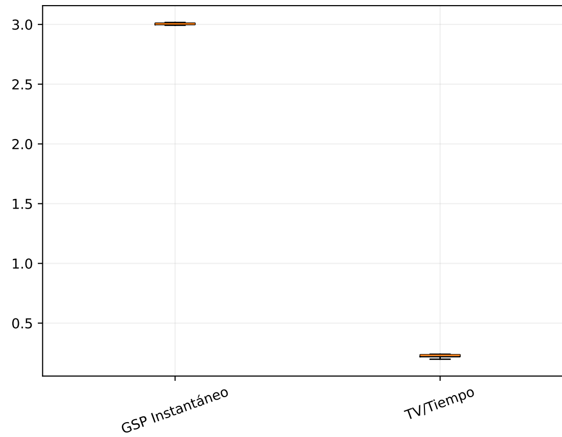
LSD
