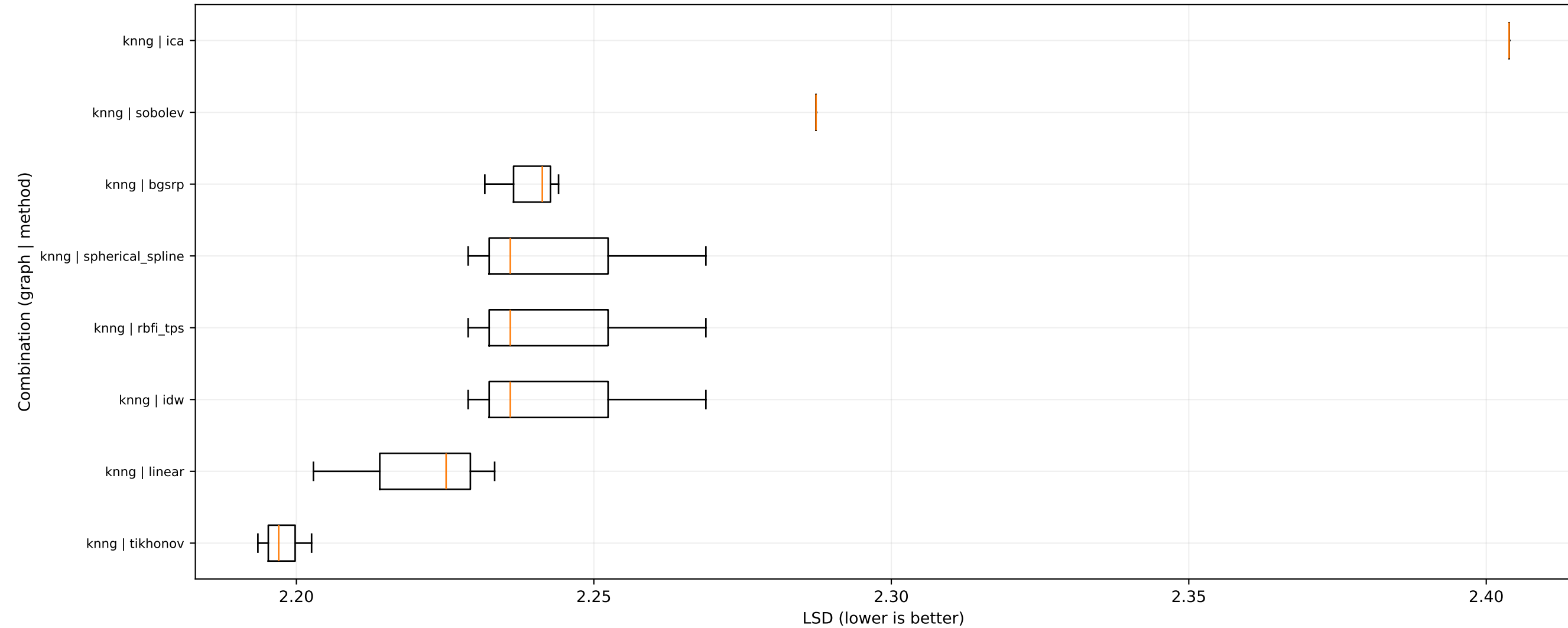
LSD distribution by graph-method combination - dataset: bci_iv2a_real_s3
