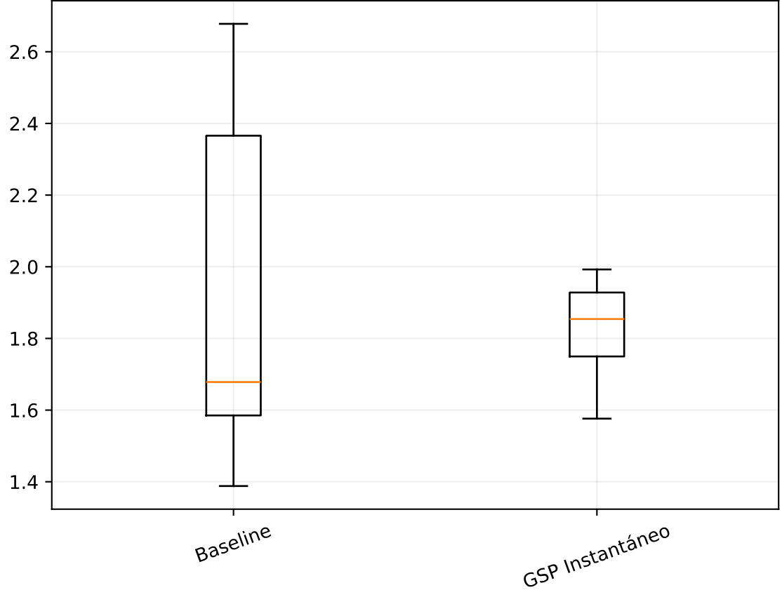
coherence_mean
