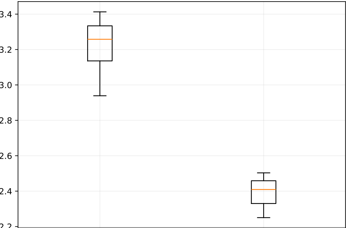
LSD
