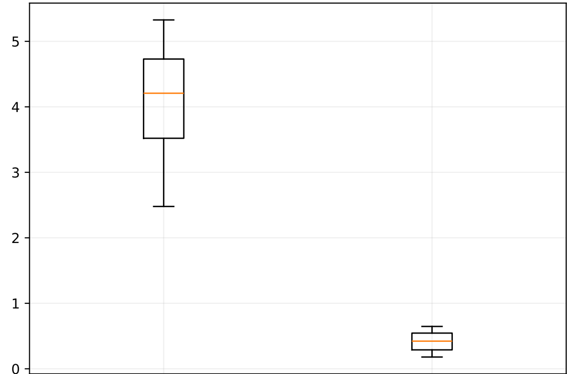
RMSE
