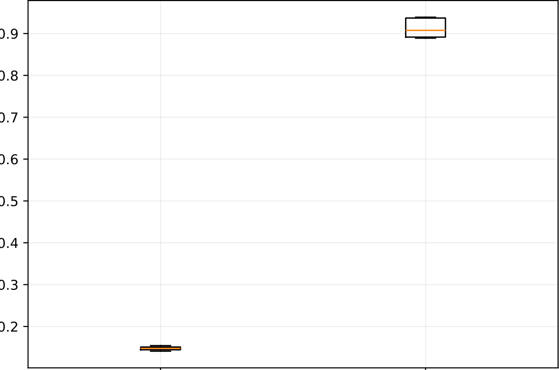
coherence_mean
