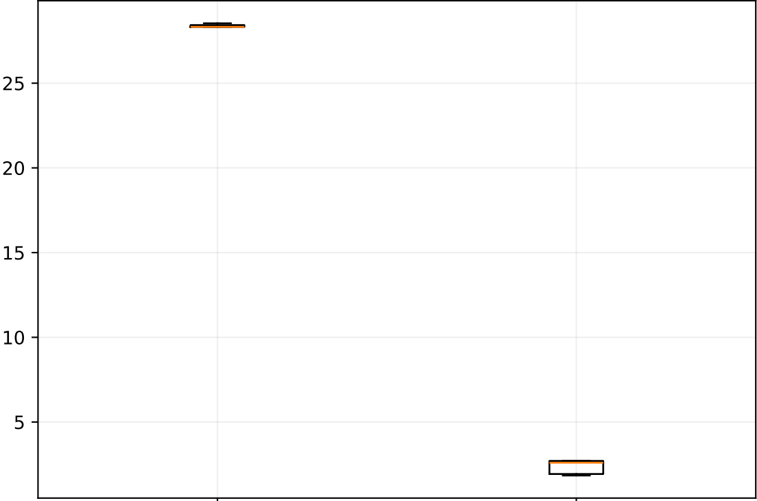
DTW
