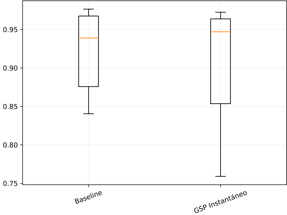
coherence_mean
