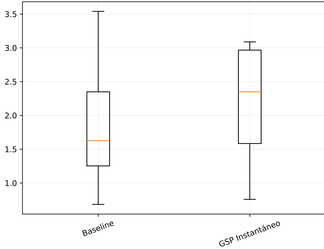
coherence_mean
