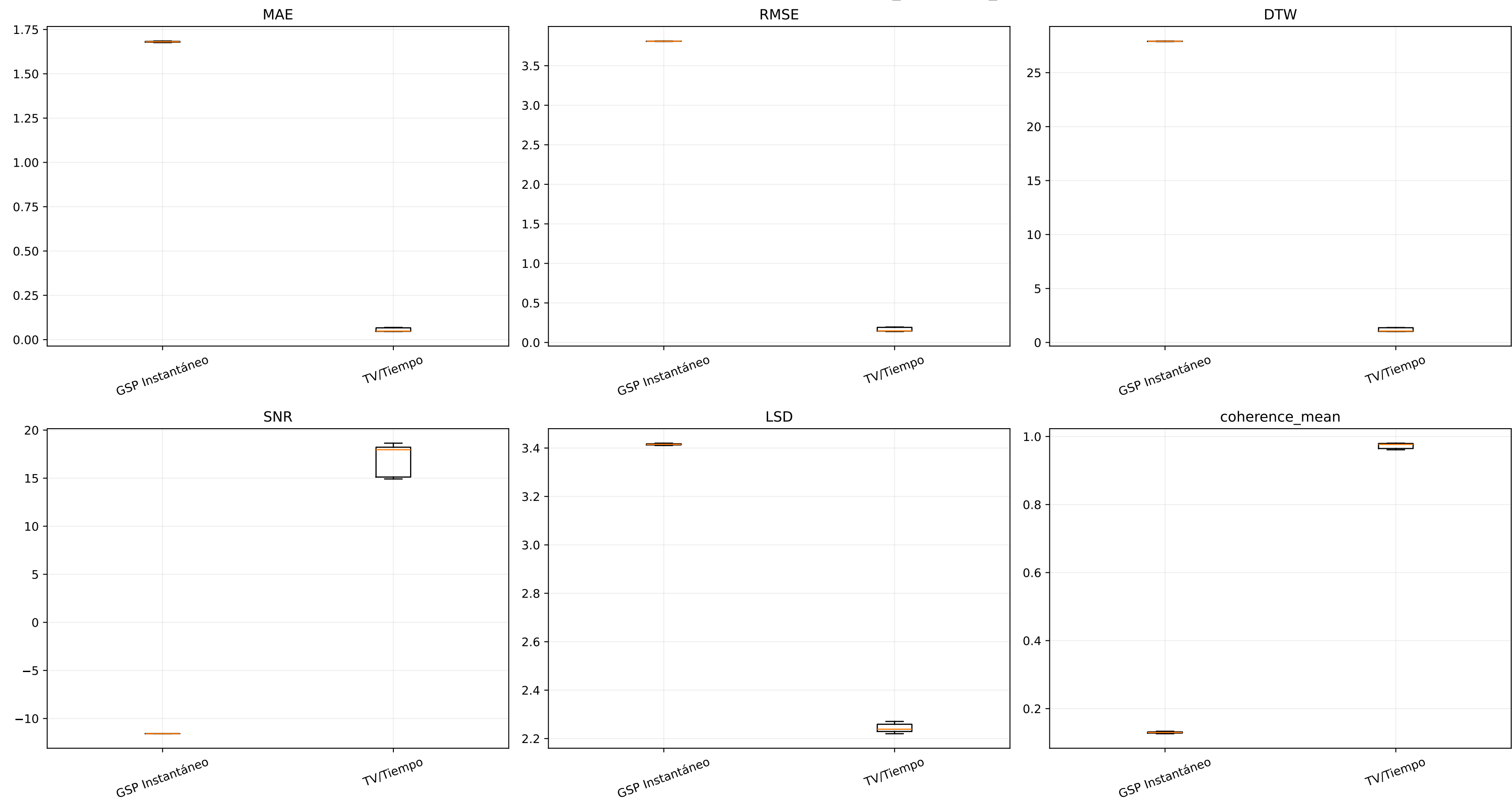
Family dispersion by metric - dataset: physionet_eegmmidb_real
