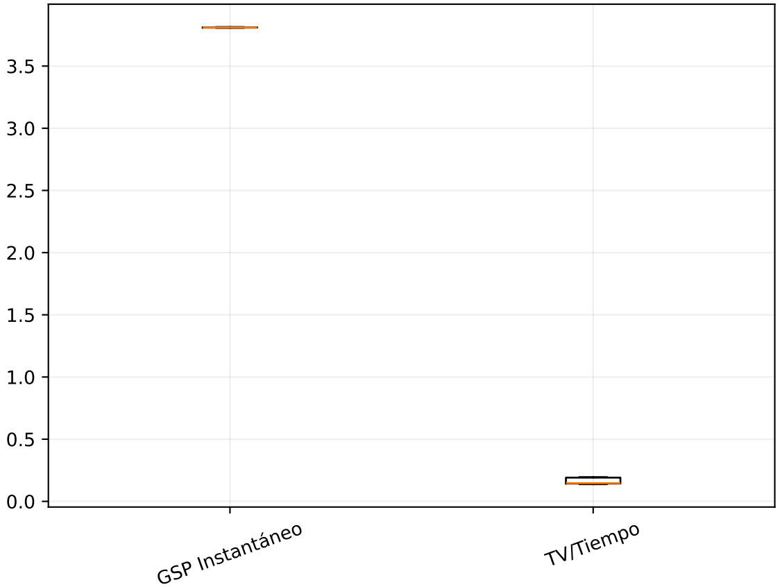
RMSE
