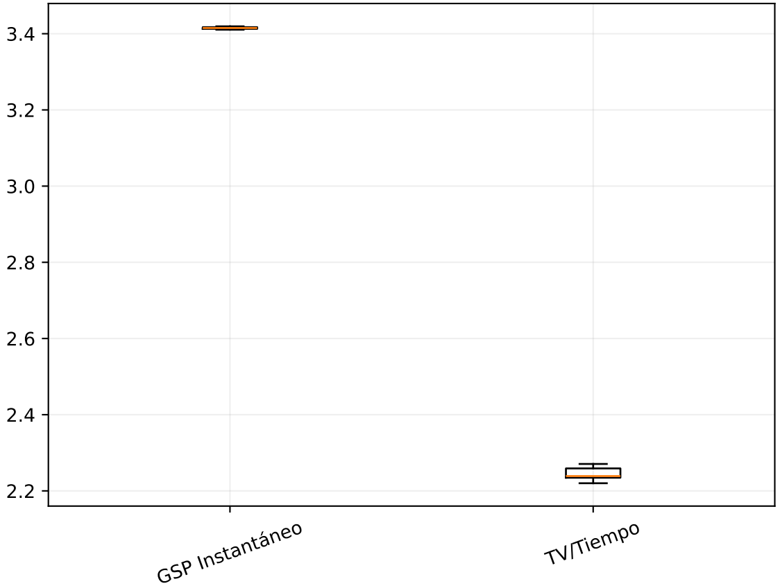
LSD
