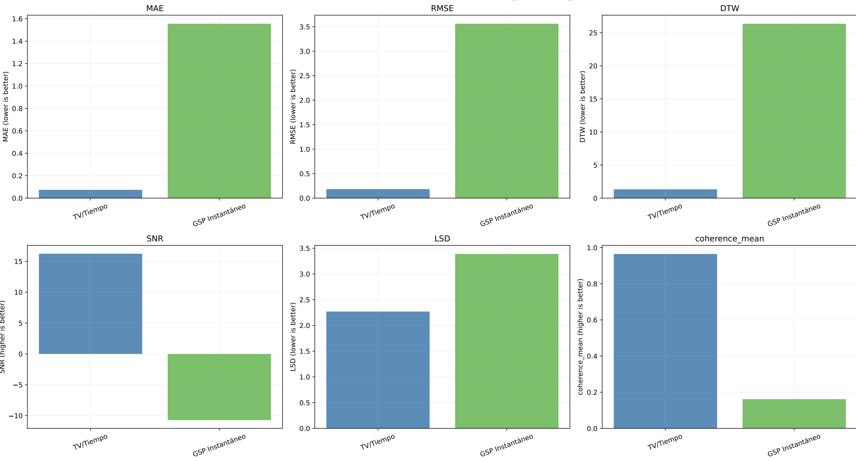
Average performance by family - dataset: physionet_eegmmidb_real
