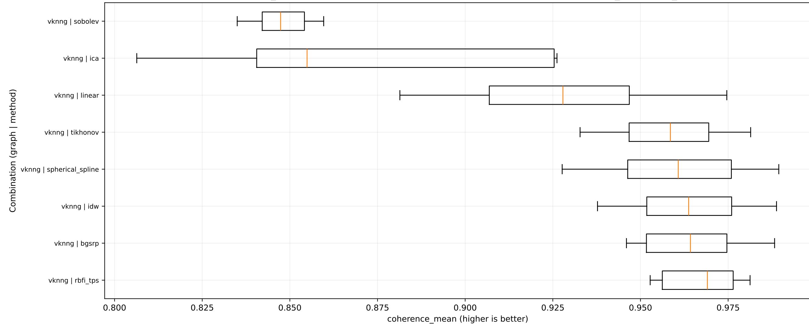
coherence_mean distribution by graph-method combination - dataset: physionet_eegmldb_real
